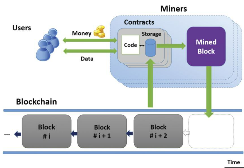
Figure 1: A blockchain-based smart contract according to [L2].
