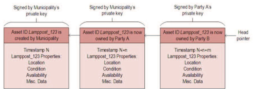
Figure 2: Simplified blockchain.
