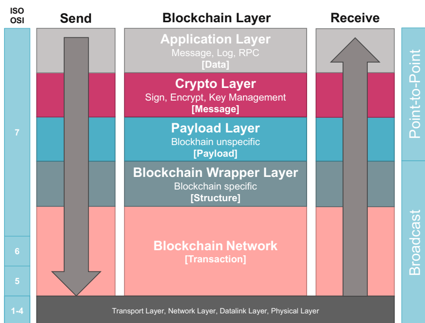
Figure 2: Usage of the blockchain in a layered architecture, in relation to the ISO-OSI model.
