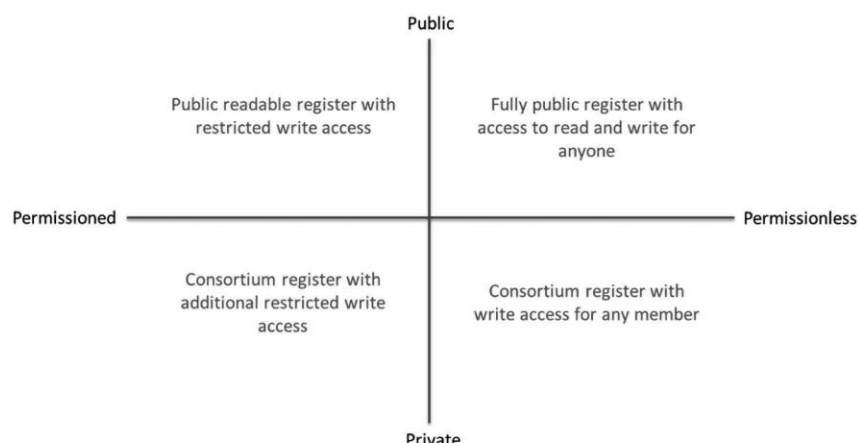
Figure 1: Types of Blockchain categorised according to read and write access [L1].
